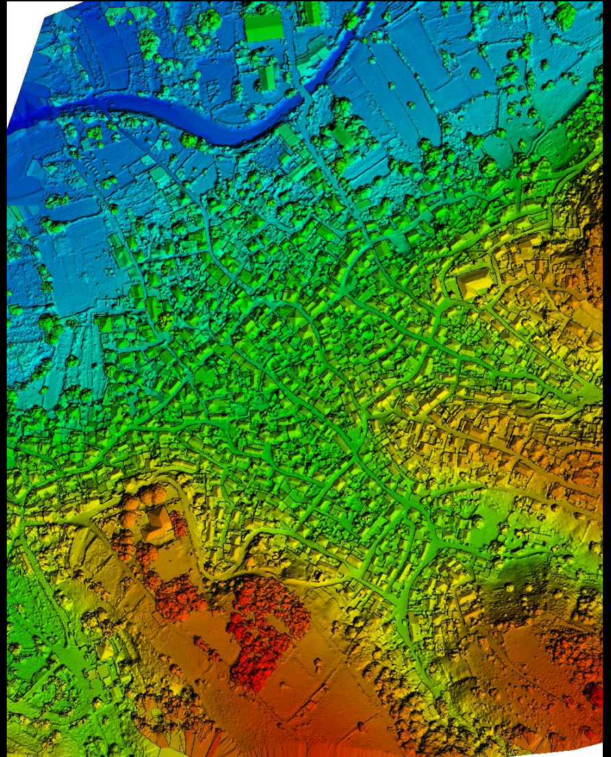
Vrissa Digital Surface Model
