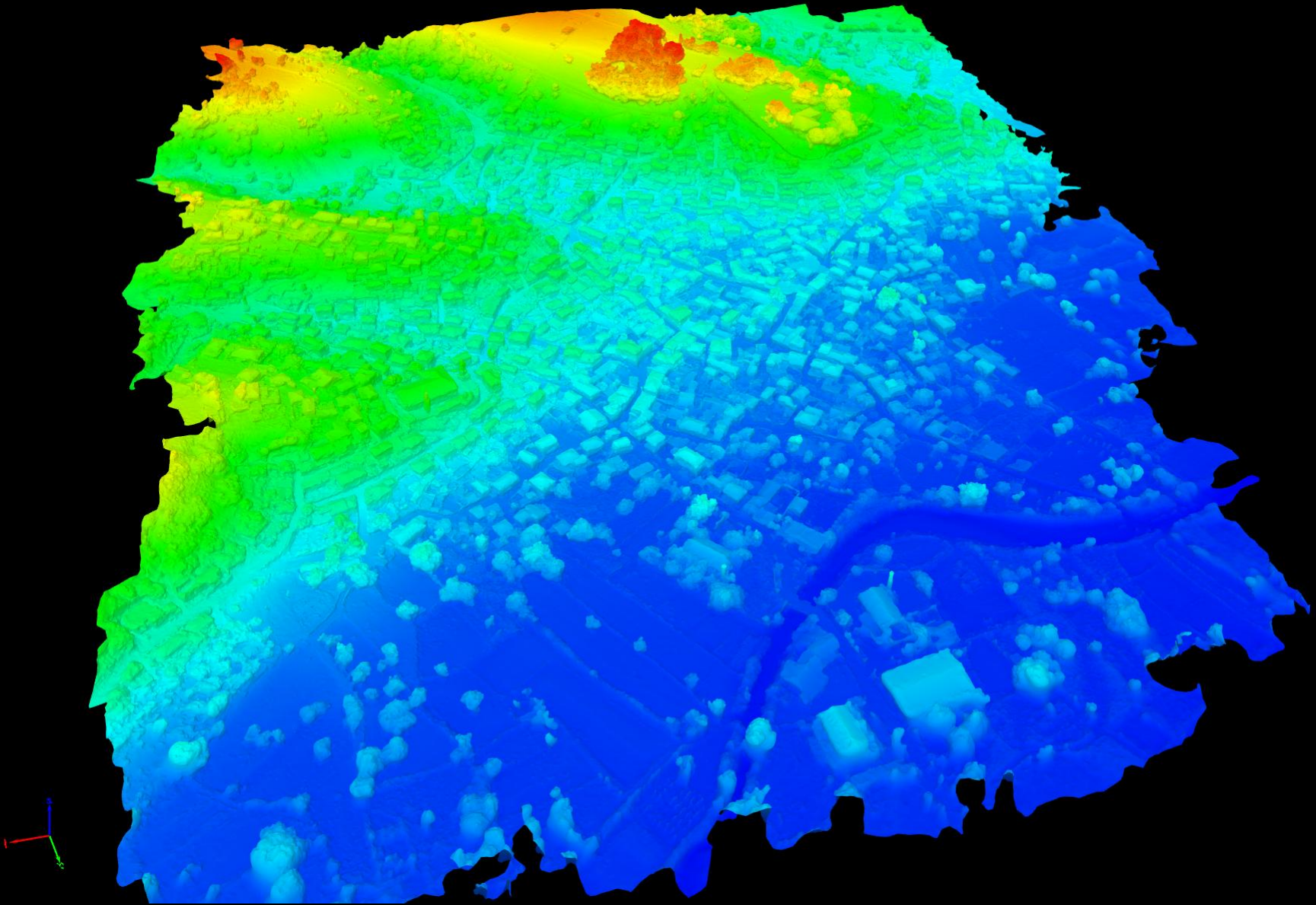
Vrissa 3D Model - Altitude
