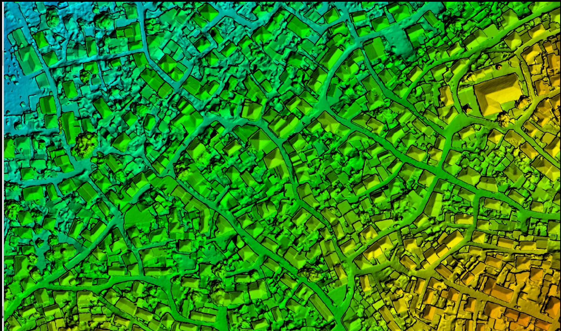
Vrissa Digital Surface Model (partial)
